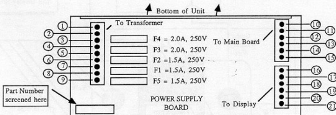
FIGURE 13 Power Supply Voltage Check points (ESQ-M)
